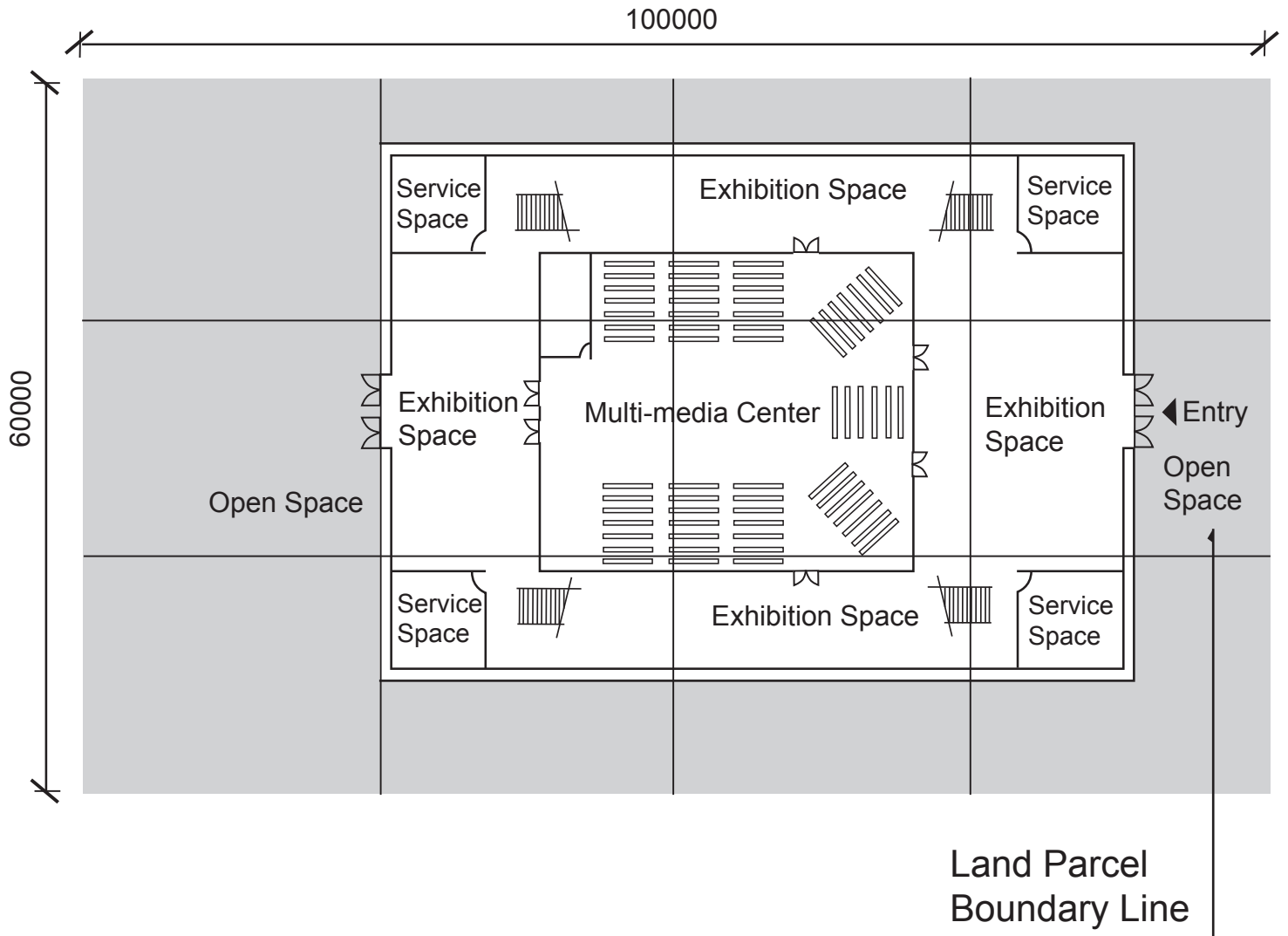
Sketch of Ground Floor Plan (unit: mm)
